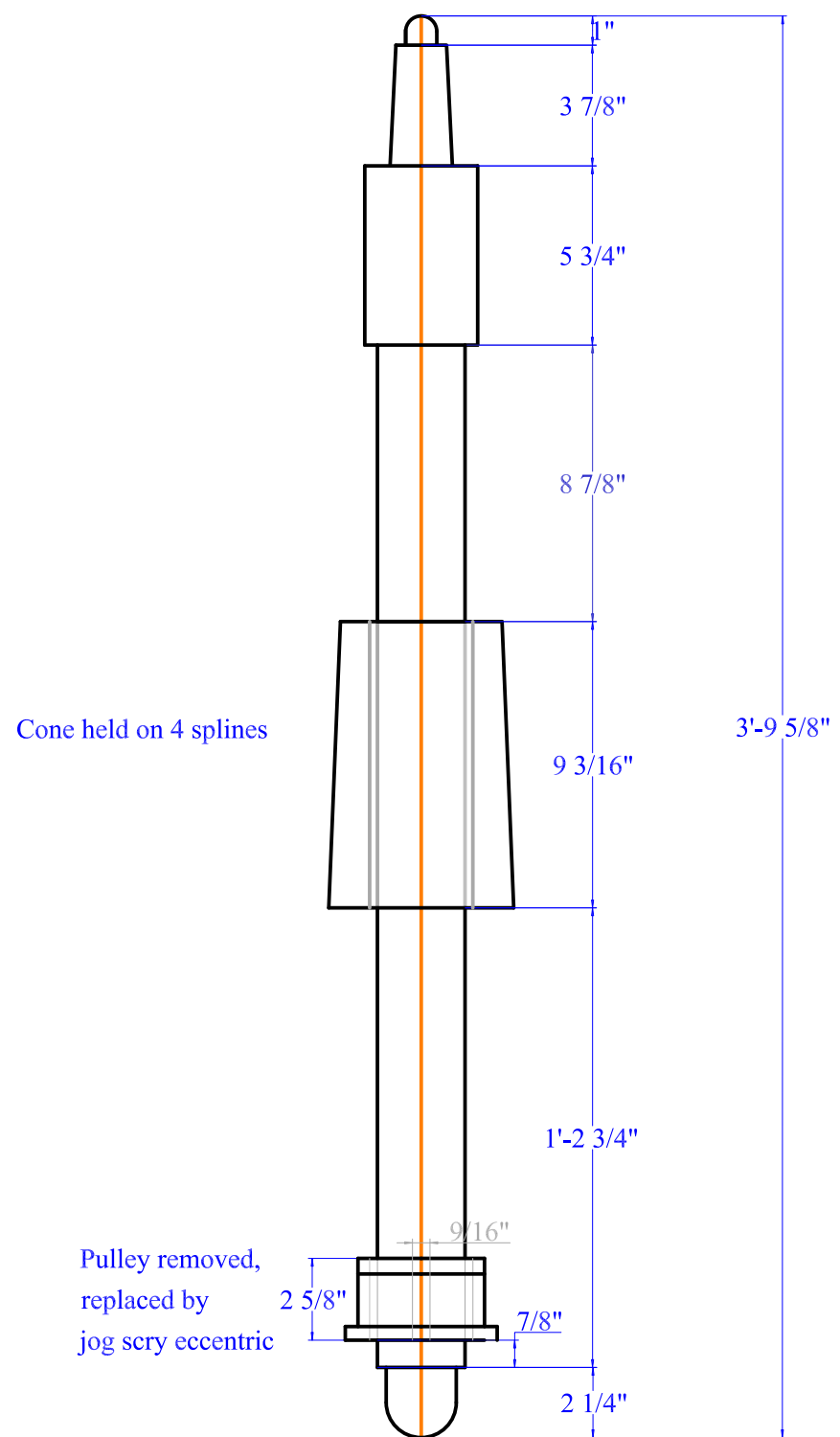
Fig 3.40 Wicken Windmill North Stone Spindle
