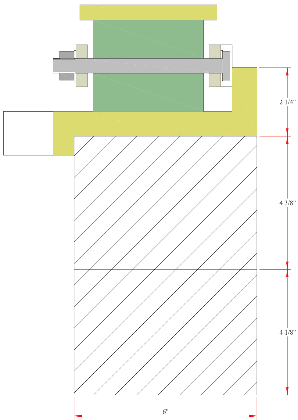
Fig 2.24 Wicken Windmill: Curb Section, Roller, Cage and Cap Runner Plate
