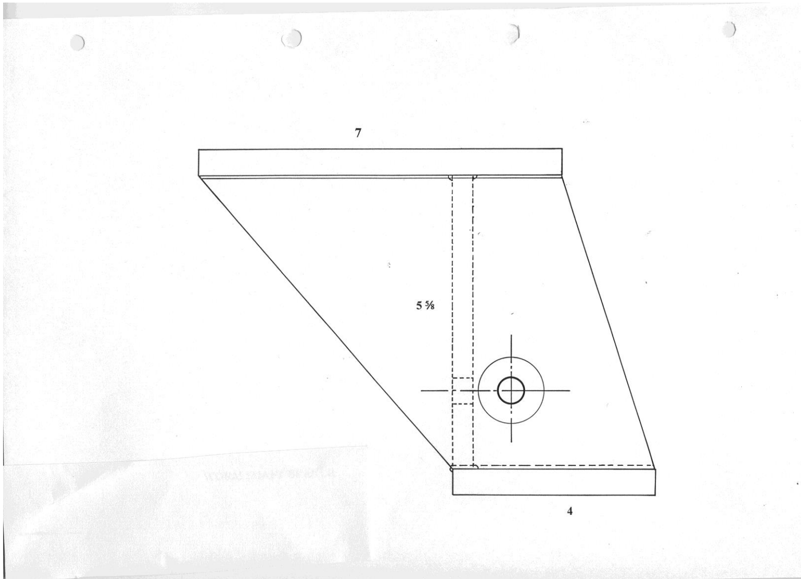
Fig 2.8 Worm Shaft Bearer, based on a drawing by A.D. Wallis
