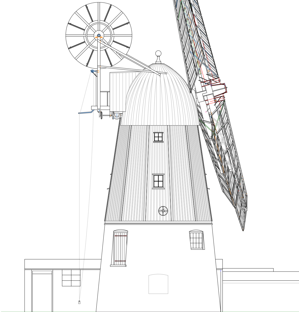
Fig 5.2 WICKEN WINDMILL: MILL & GRANARY
