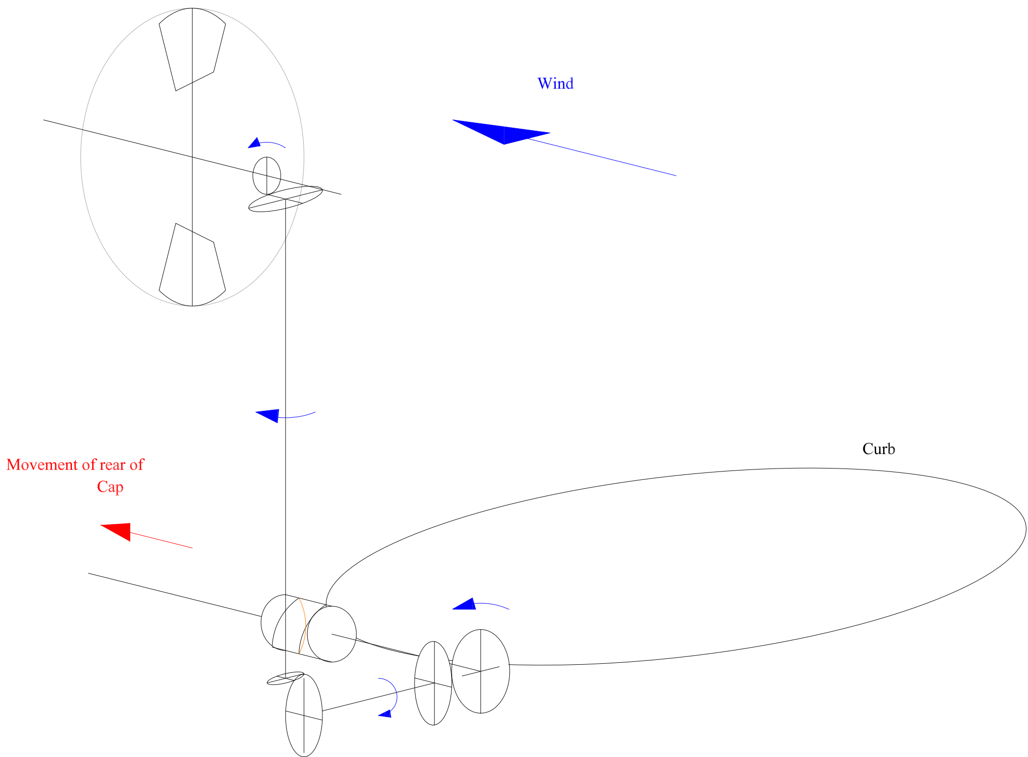
Fig 2.12 Wicken Windmill: Fan Drive layout
