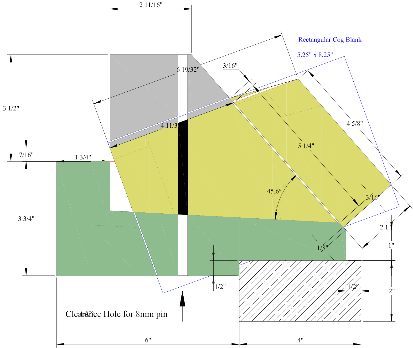
Fig 3.11a Wicken Windmill: new waller - bevelled cog & blank
