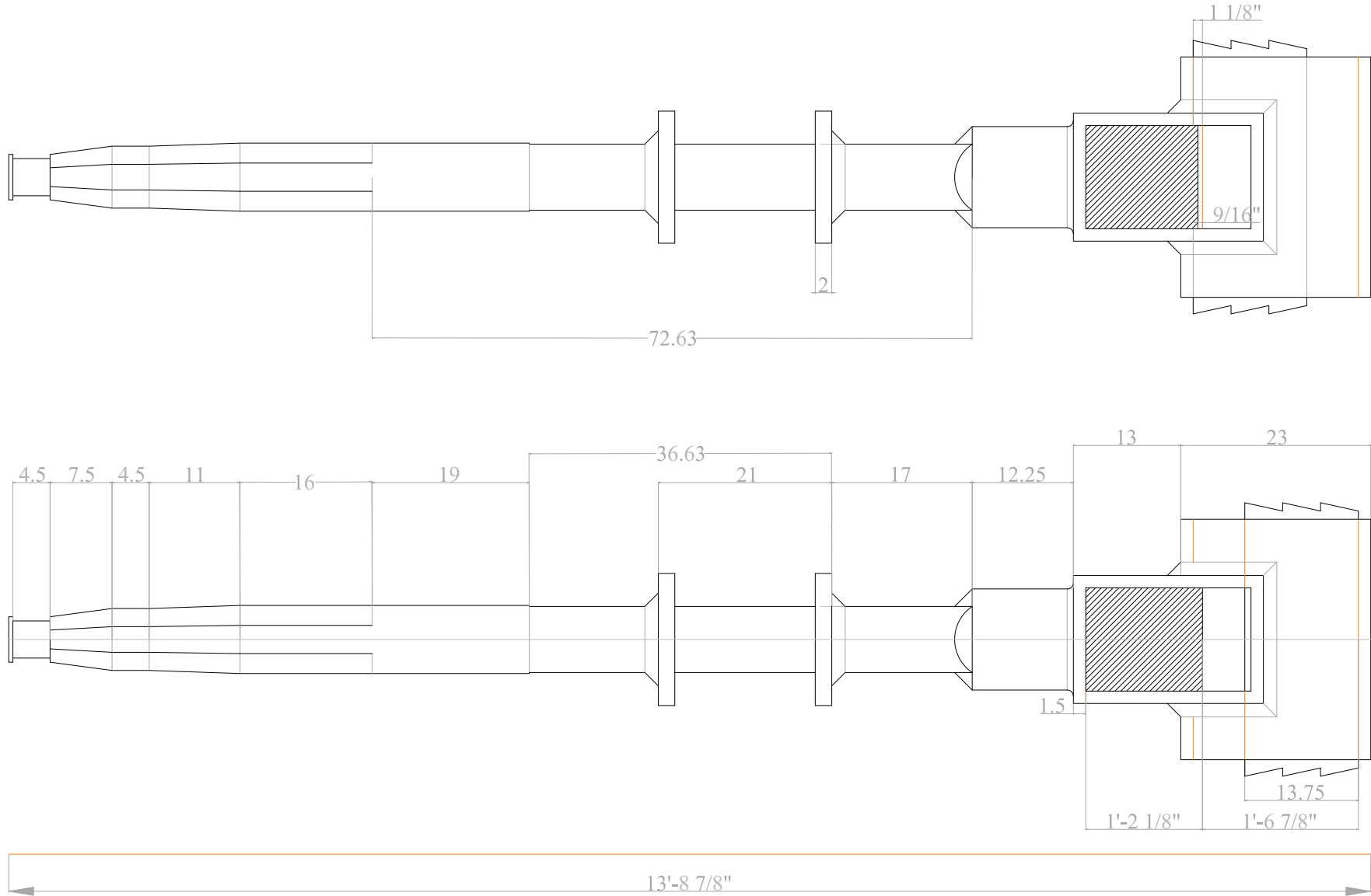
Fig 1.20 Wicken Windmill: windshaft, and stock fitting options
