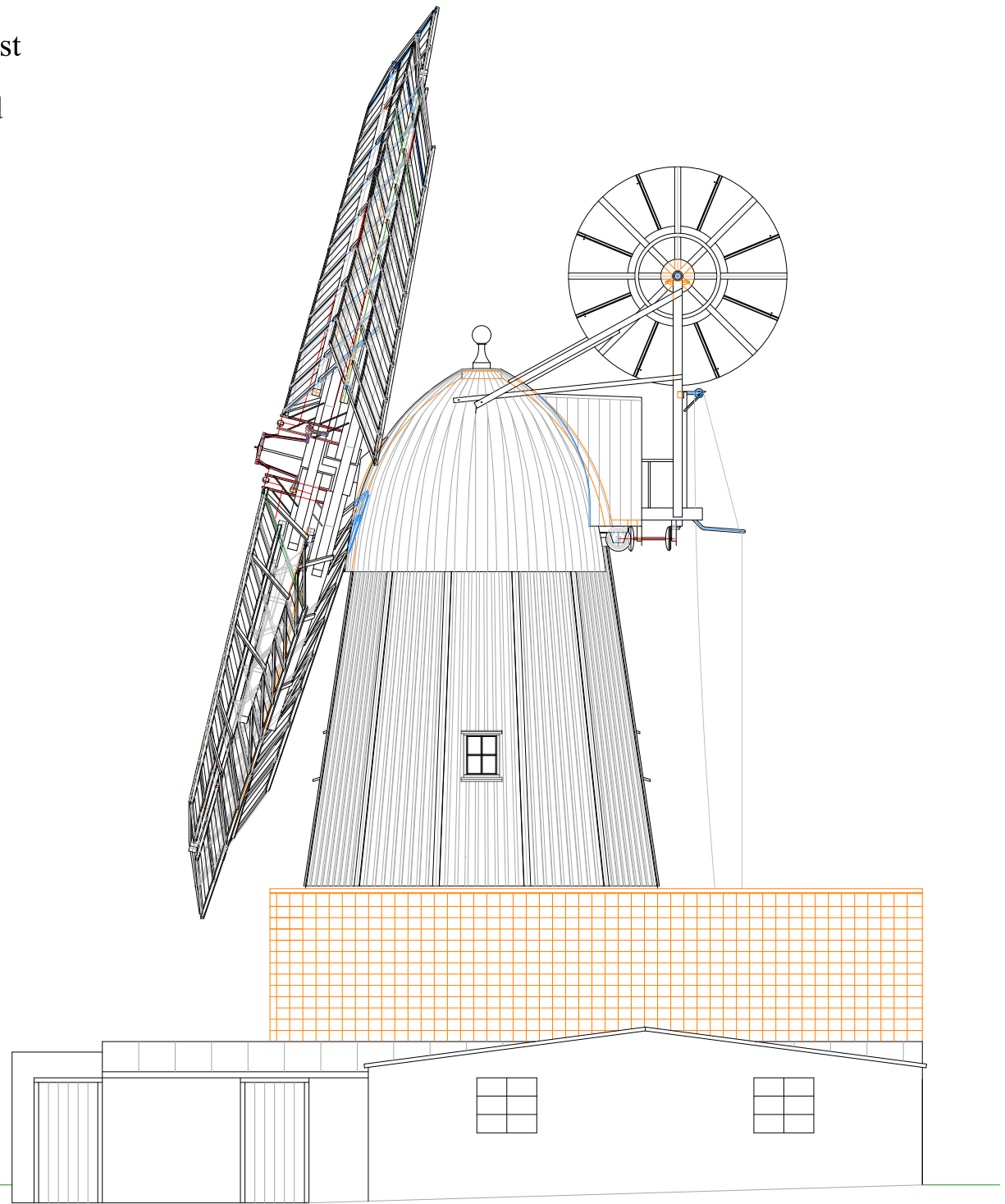
Fig 5.5 WICKEN MILLS: WINDMILL & GRANARY Proposed reinstatement of Granary roofs
