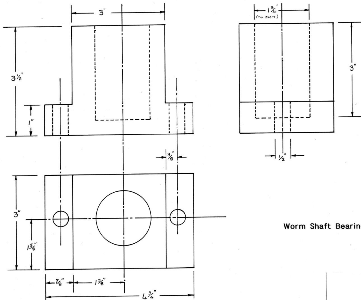
Fig 2.10a Worm Shaft Bearing, left hand, taken from a drawing by A.D. Wallis
