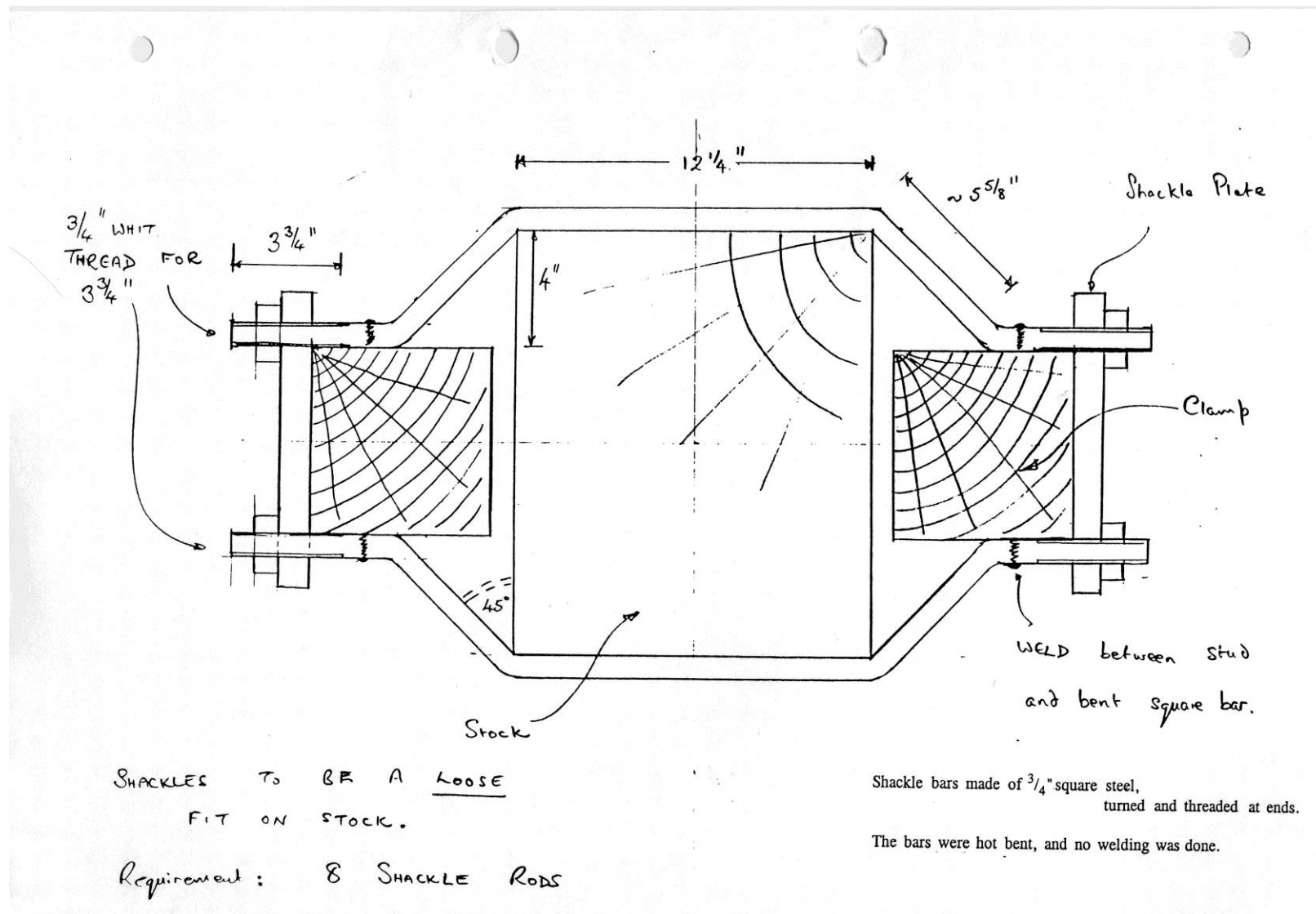
Fig 1.9 Wicken Corn Windmill: Clamp Shackles
