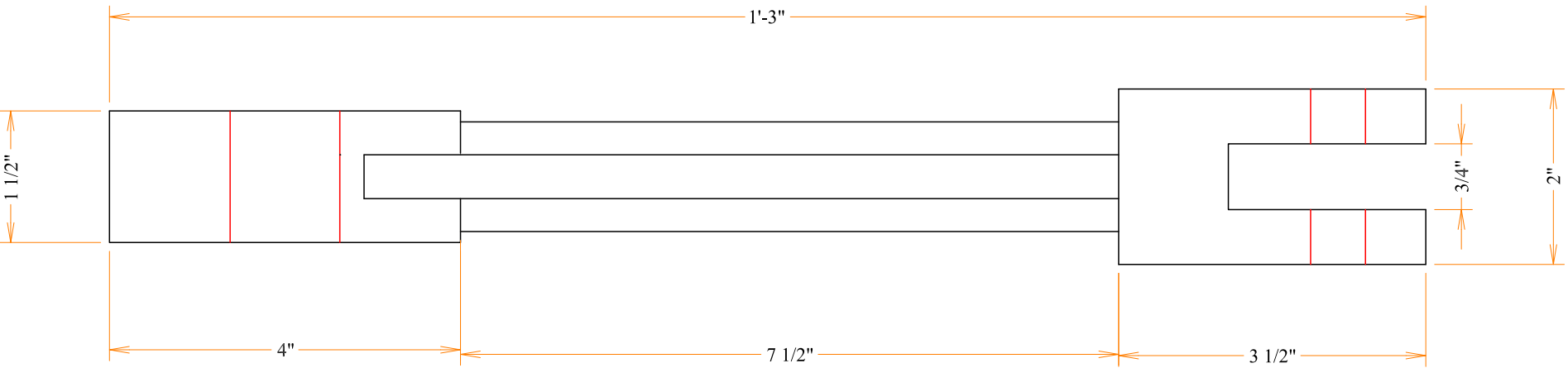
Wicken Windmill Fig 1.31 Striking Lever CastAluminium Scale: 1/2 Full Size Drawn: D.L. Pearce
