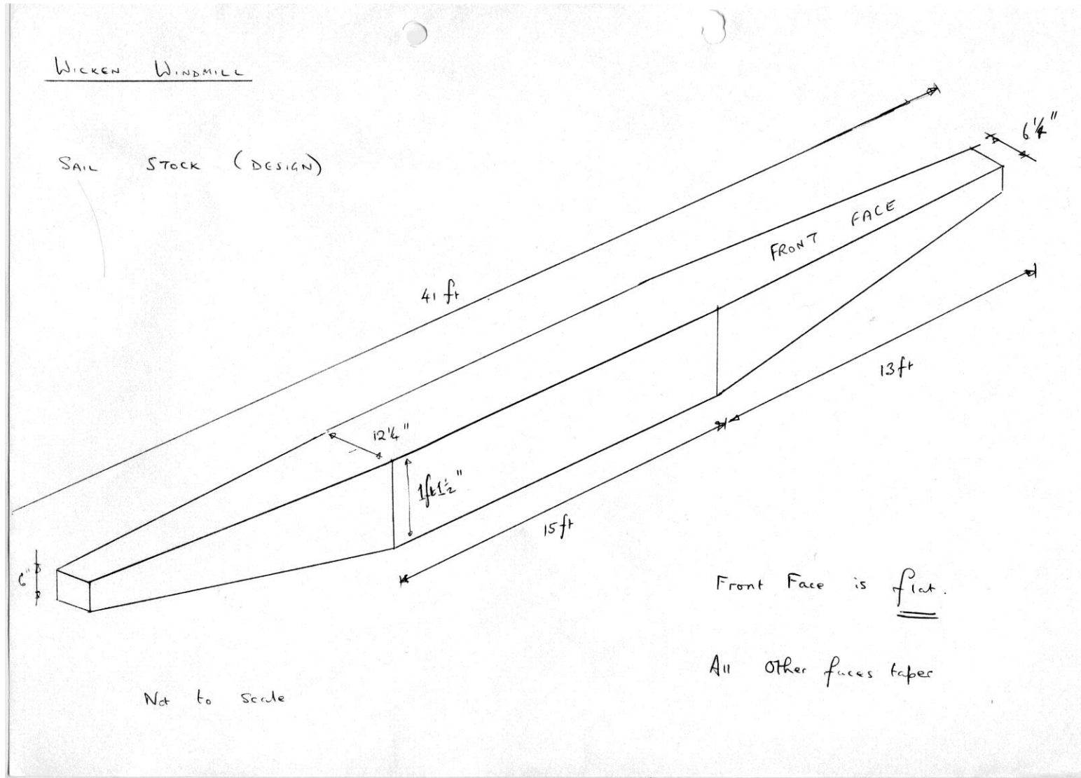
Fig 1.4 Major Sail Components: Early sketch of Sail Stock
