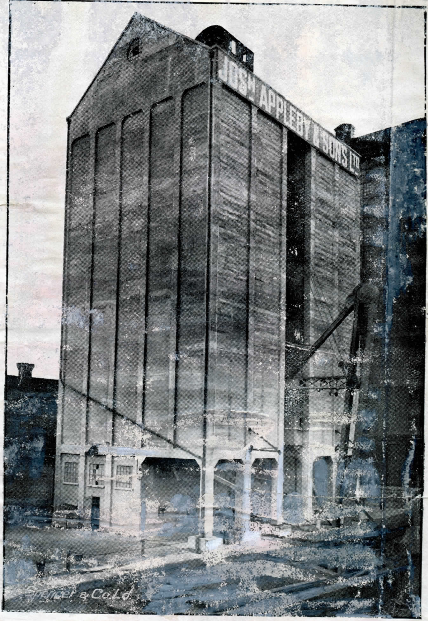
Ferro-concrete Silo for Grain at Liverpool
